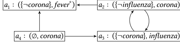
Figure 5: The AF F(K_{\text{covid}^*}^* \cup \{\text{fever} \wedge \text{short-of-breath}\}, A) .
