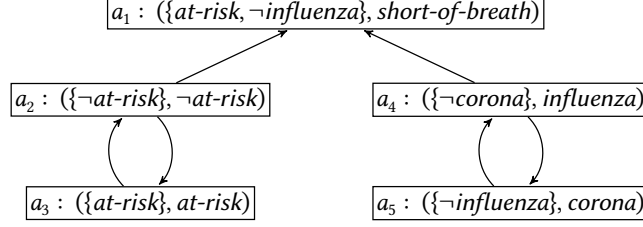
Figure 2: The AF F(K \cup \{\text{fever}\}, A) .
