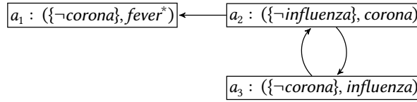
Figure 4: The AF F((K_{covid^*=\perp}^* \cup \{fever\}, A) .
